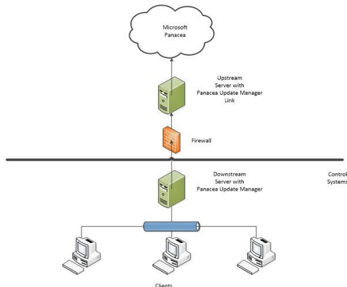
Figure 1: Example Mixed Mode Architecture
